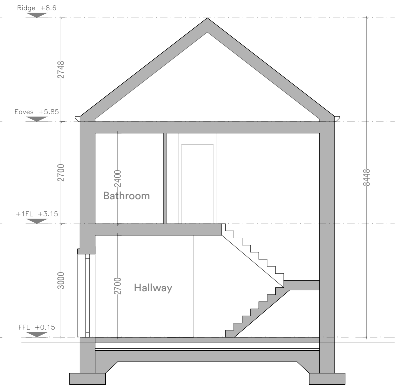
House Type R2 Detached Section A.A
